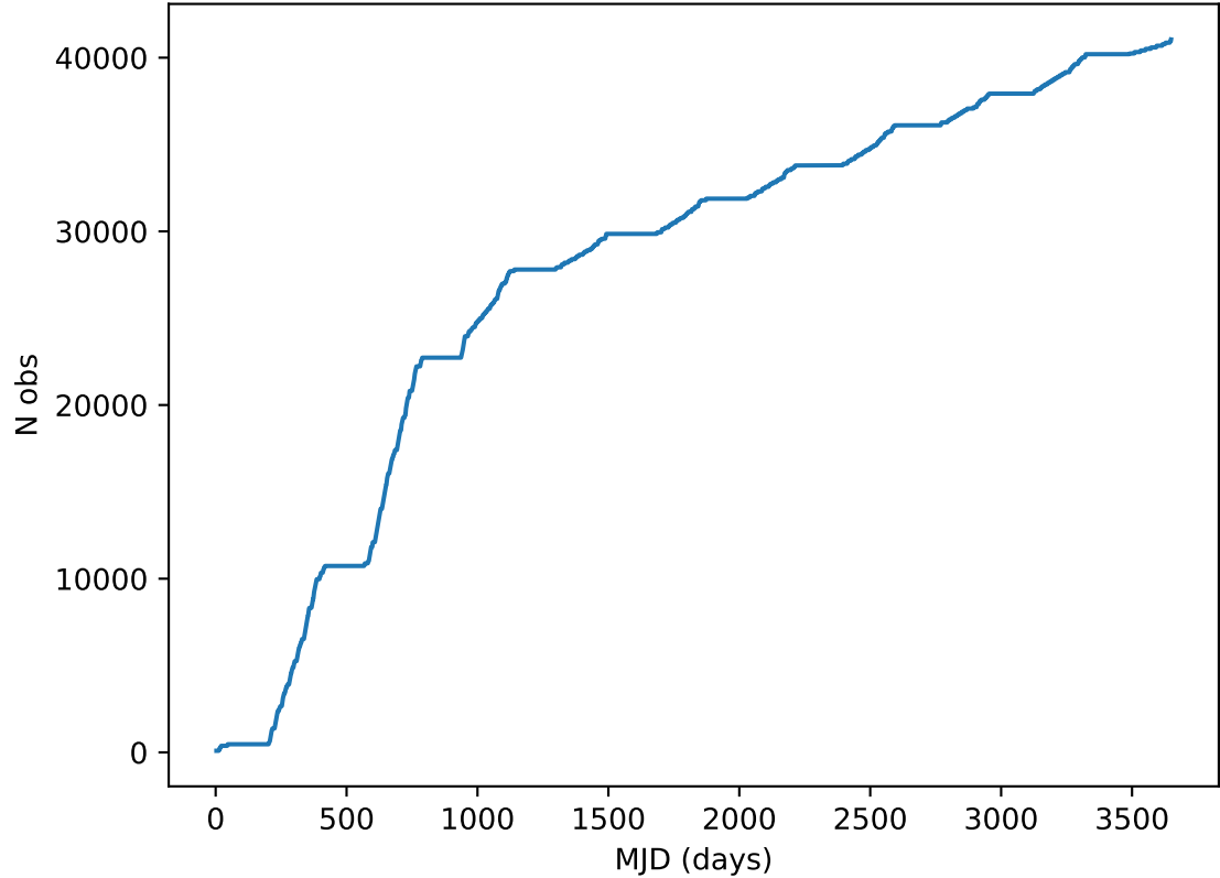
roll_uniform_early_half_accordion1_mjdp0_v3.4_10yrs all bands: DD:COSMOS Cumulative NVisits
