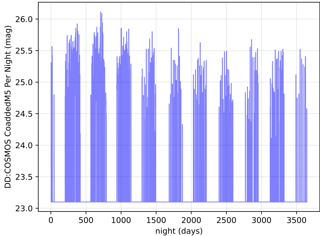
roll_uniform_early_half_accordion1_mjdp0_v3.4_10yrs i band: DD:COSMOS CoaddedM5 Per Night
