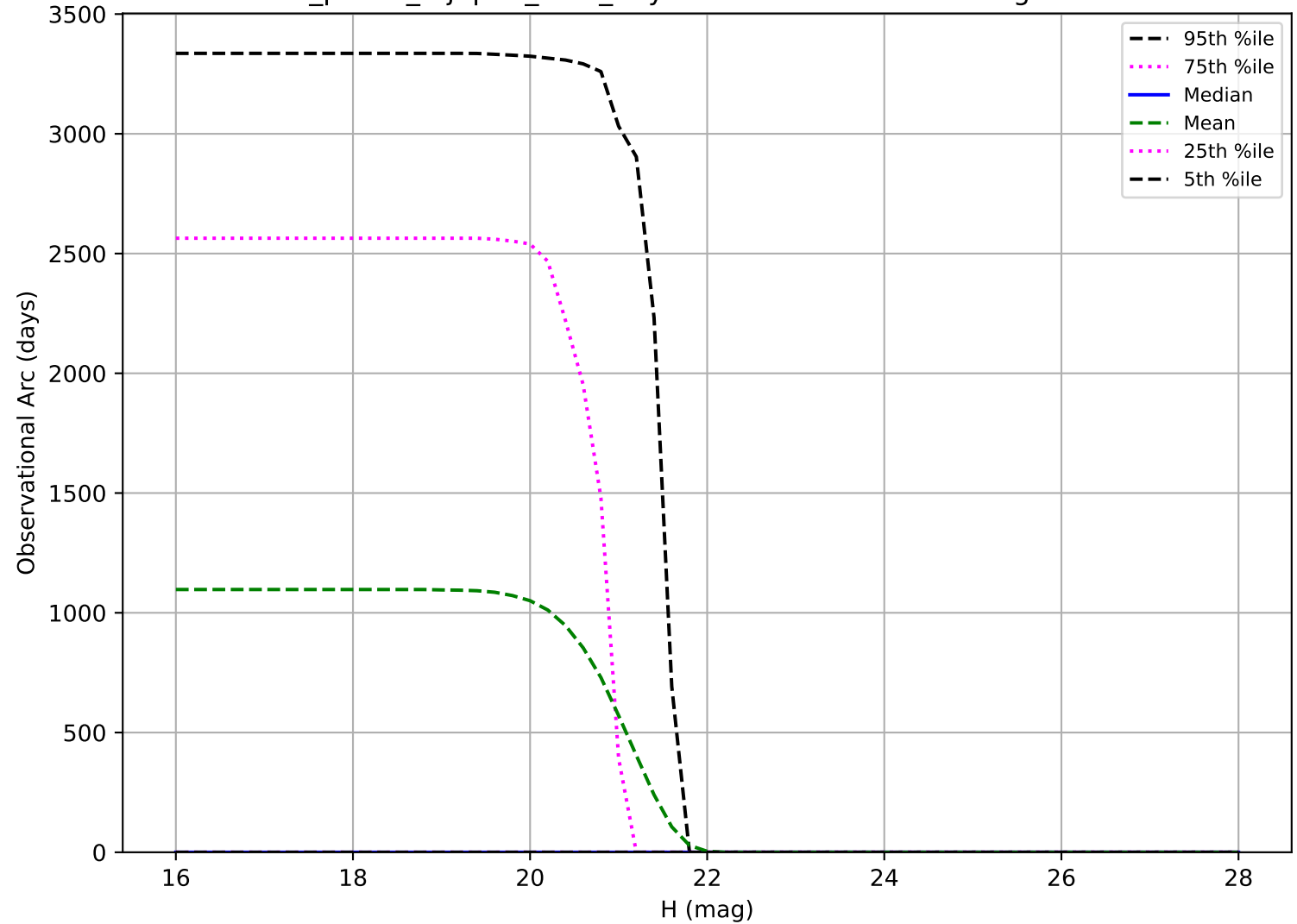
roll_pause_mjdp60_v3.4_10yrs: Observational Arc Length Vatra
