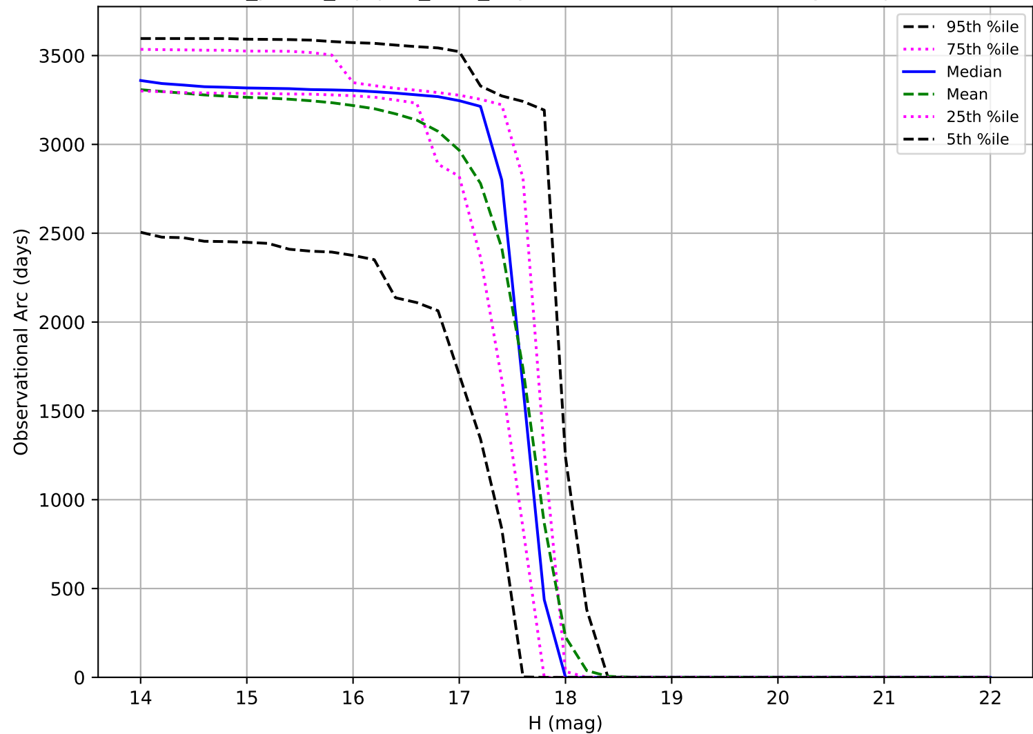
roll_pause_mjdp60_v3.4_10yrs: Observational Arc Length Trojan
