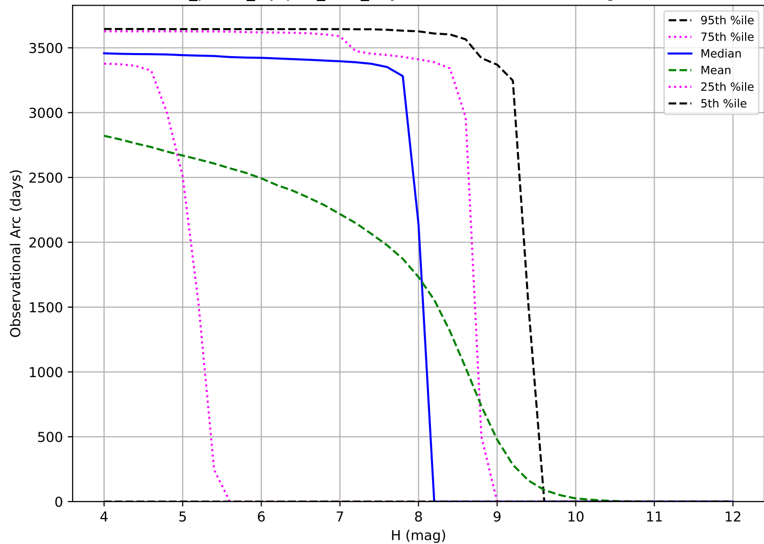
roll_pause_mjdp60_v3.4_10yrs: Observational Arc Length TNO
