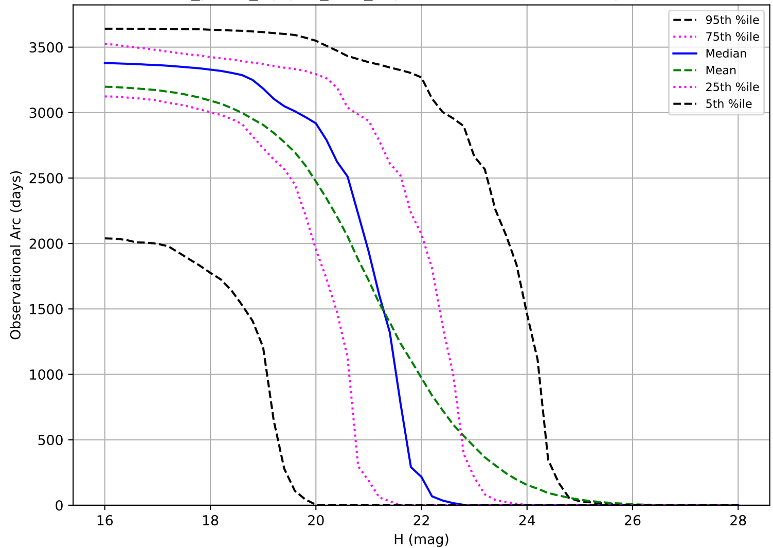
roll_pause_mjdp60_v3.4_10yrs: Observational Arc Length PHA
