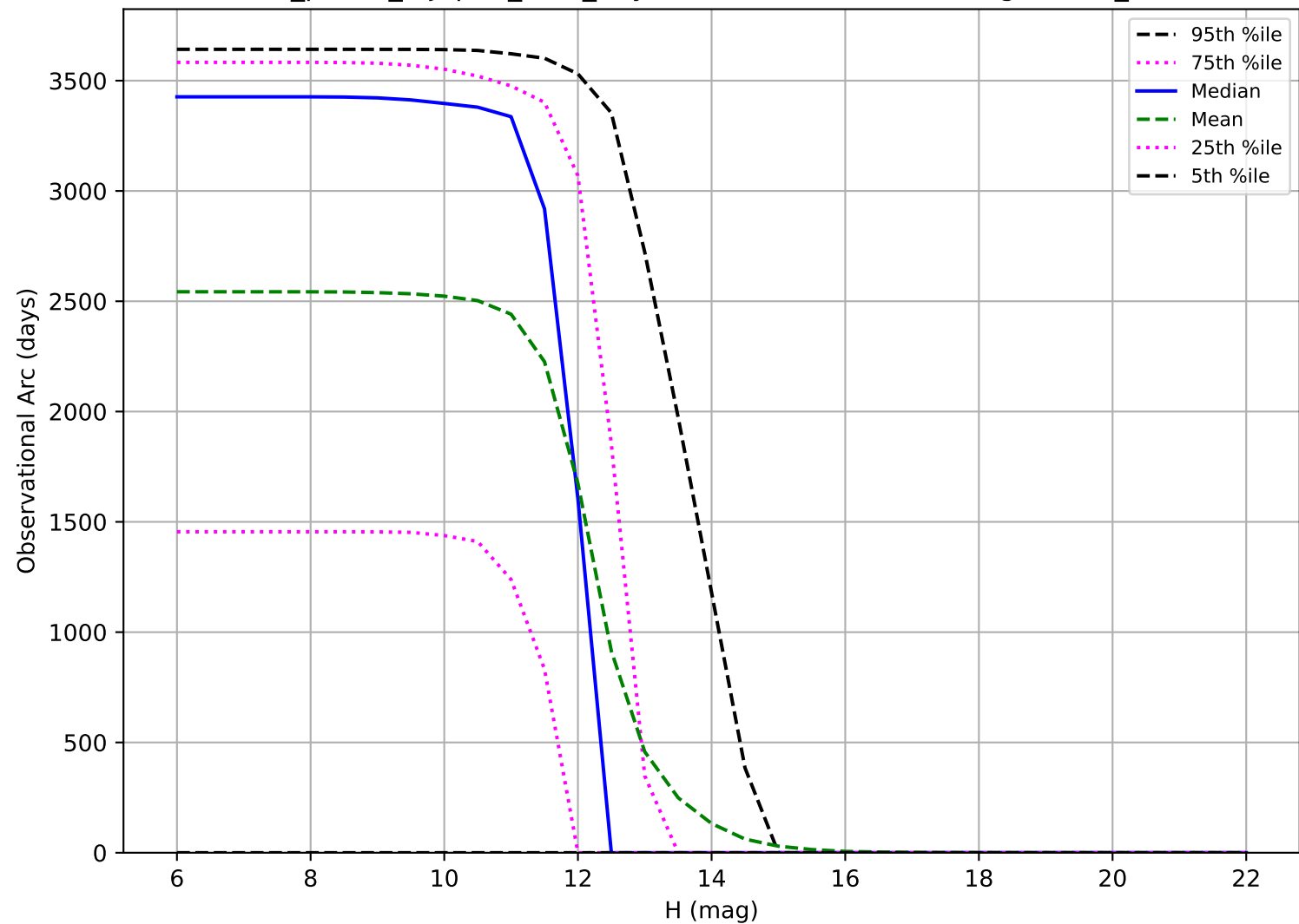
roll_pause_mjdp60_v3.4_10yrs: Observational Arc Length OCC_r20
