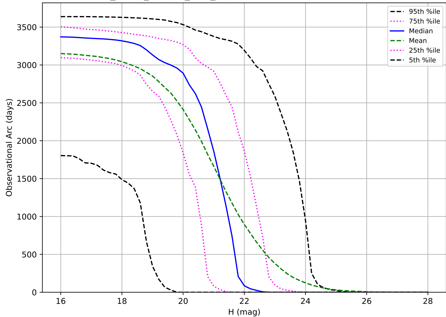
roll_pause_mjdp60_v3.4_10yrs: Observational Arc Length NEO
