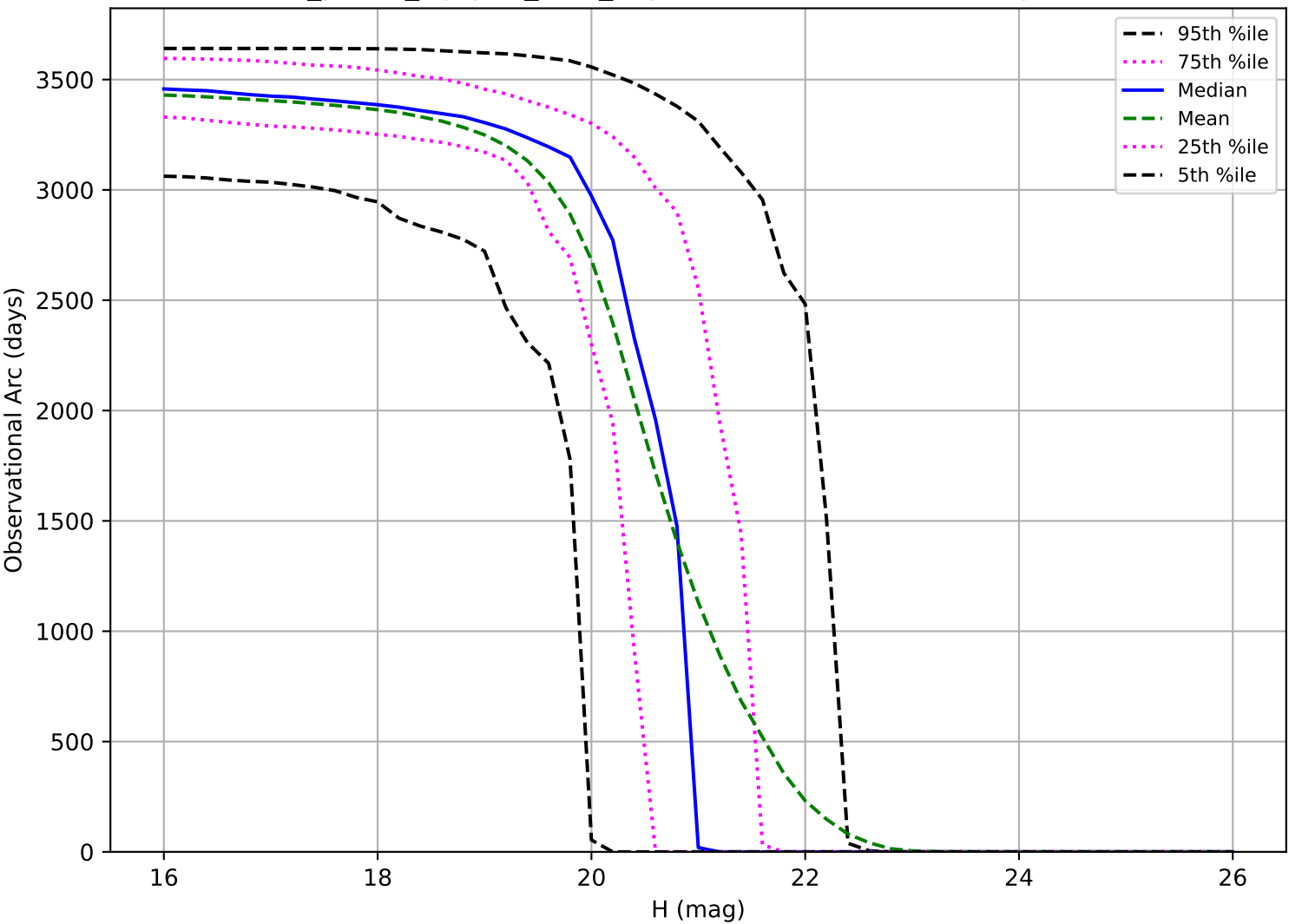
roll_pause_mjdp60_v3.4_10yrs: Observational Arc Length MBA
