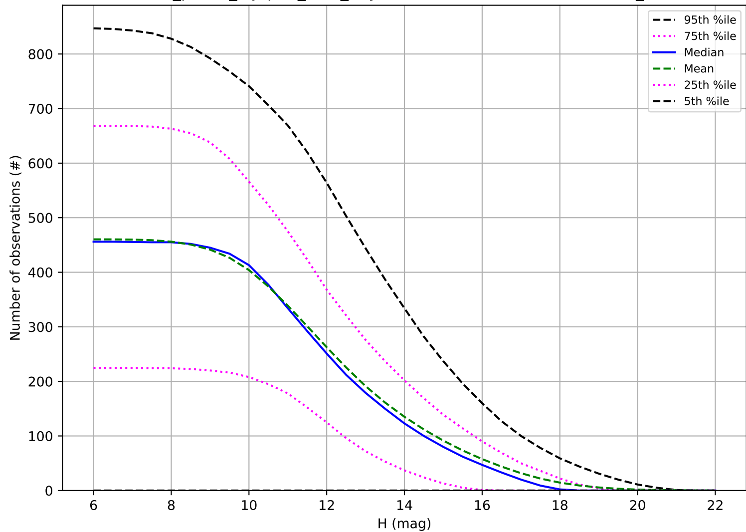
roll_pause_mjdp60_v3.4_10yrs: Number of observations OCC_r5
