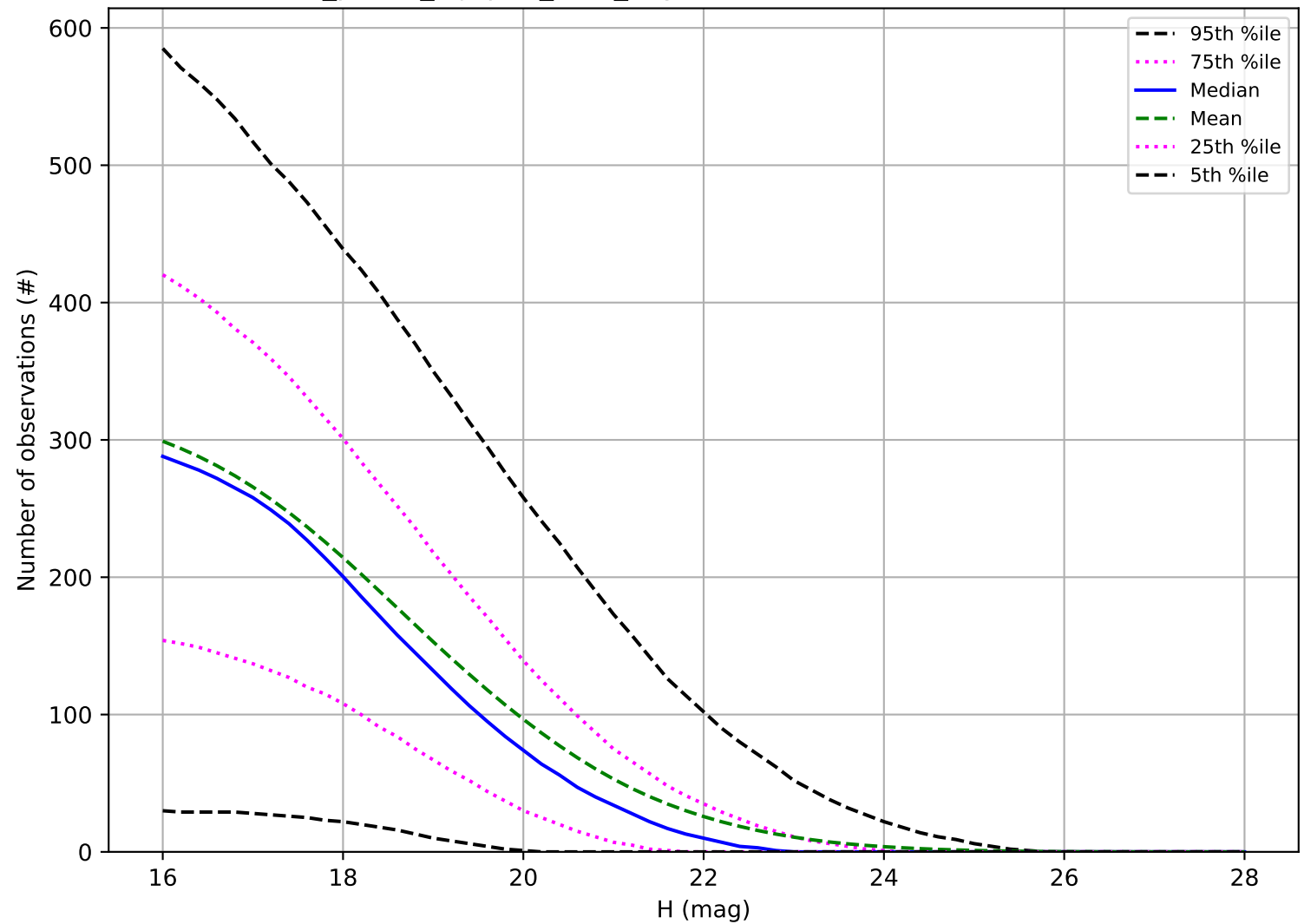
roll_pause_mjdp60_v3.4_10yrs: Number of observations NEO
