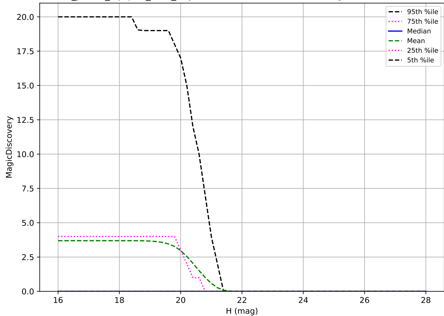
roll_pause_mjdp60_v3.4_10yrs: Vatira 6 detections in 60 nights detection loss
