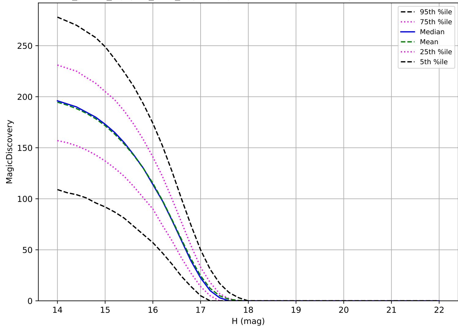
roll_pause_mjdp60_v3.4_10yrs: Trojan 6 detections in 60 nights detection loss
