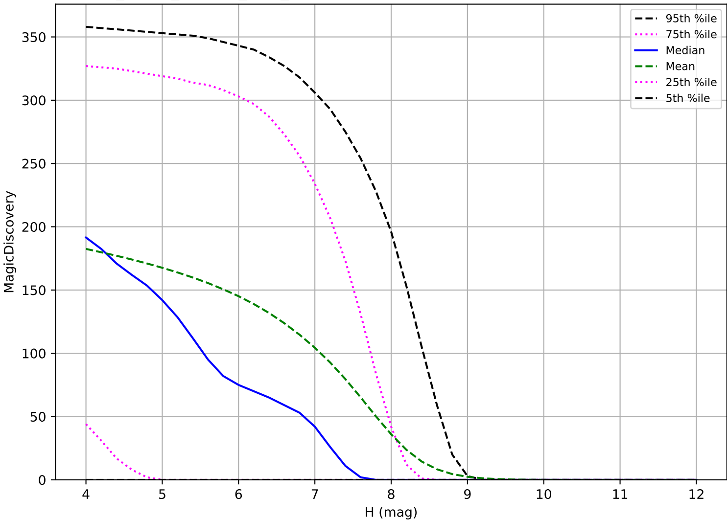
roll_pause_mjdp60_v3.4_10yrs: TNO 6 detections in 60 nights detection loss
