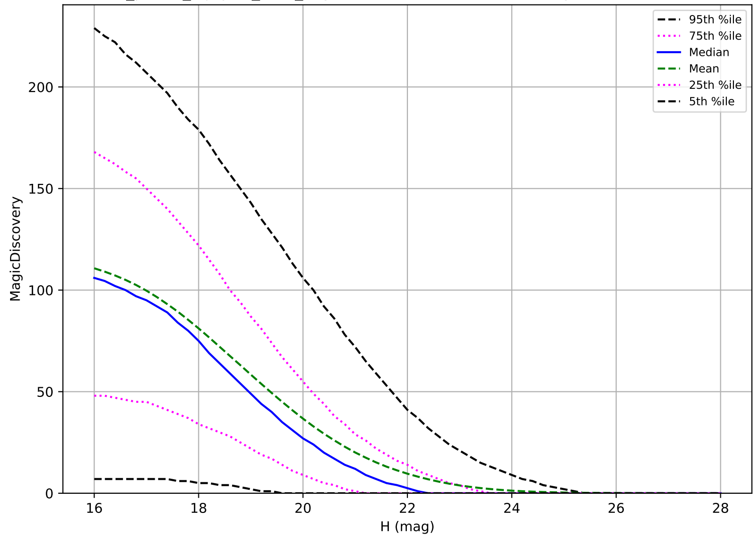
roll_pause_mjdp60_v3.4_10yrs: PHA 6 detections in 60 nights detection loss
