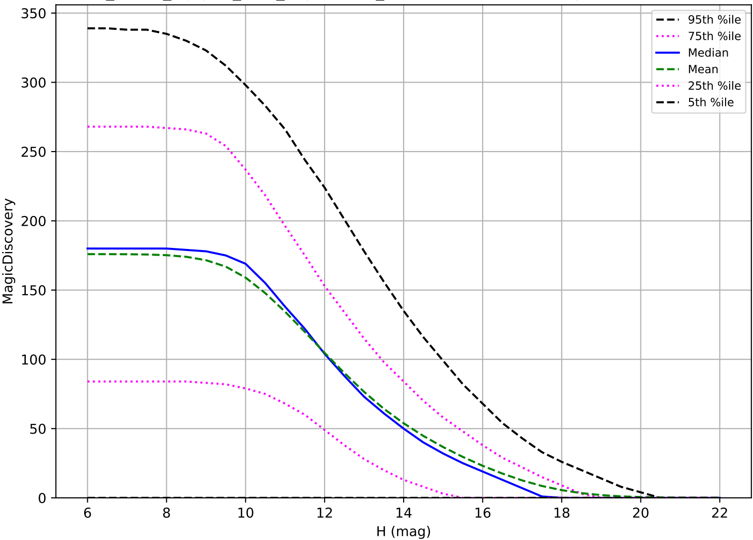
roll_pause_mjdp60_v3.4_10yrs: OCC_r5 6 detections in 60 nights detection loss
