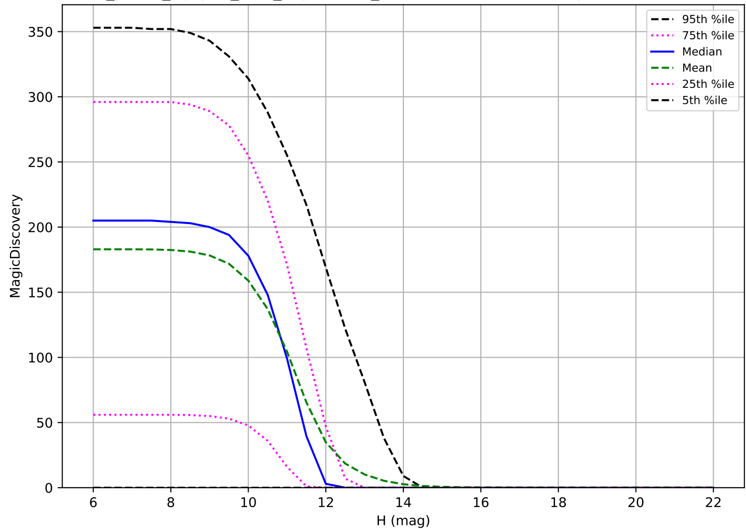
roll_pause_mjdp60_v3.4_10yrs: OCC_r20 6 detections in 60 nights detection loss
