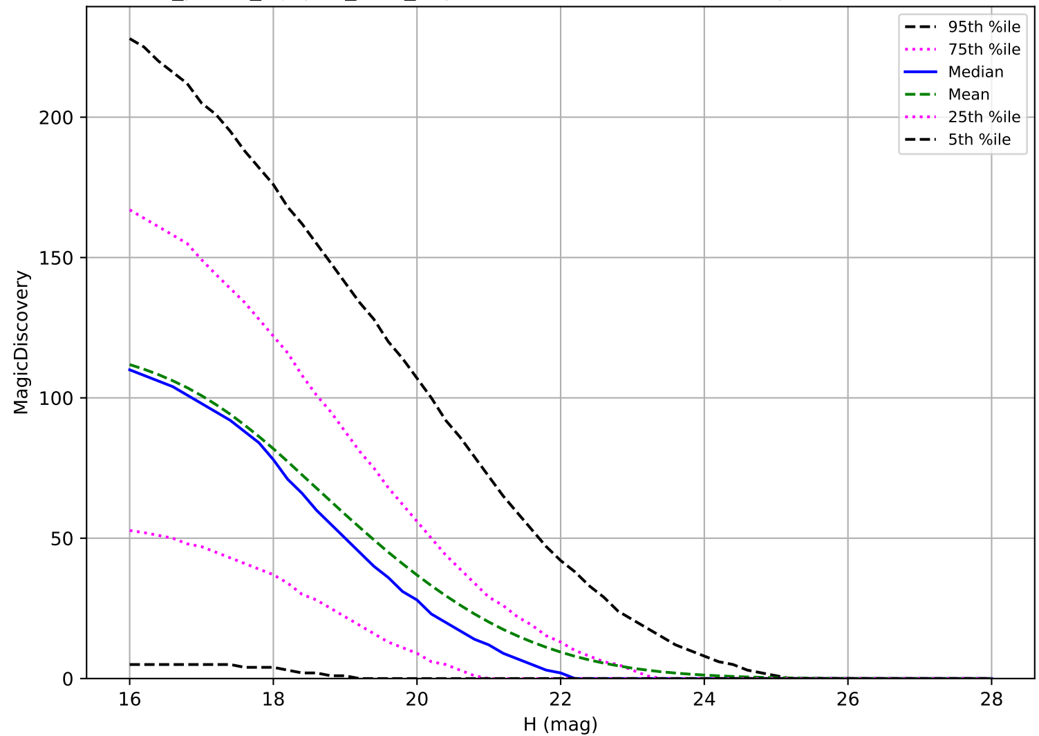
roll_pause_mjdp60_v3.4_10yrs: NEO 6 detections in 60 nights detection loss
