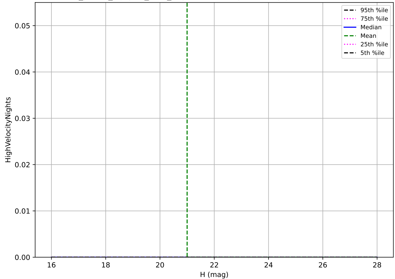
roll_pause_mjdp60_v3.4_10yrs: Vatira High velocity pair detection loss
