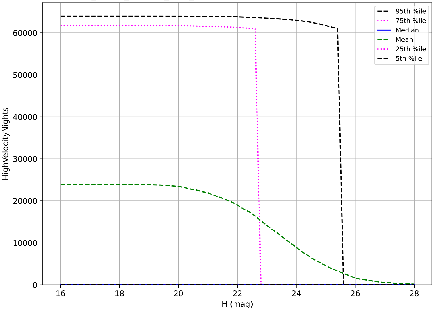
roll_pause_mjdp60_v3.4_10yrs: PHA High velocity pair detection loss
