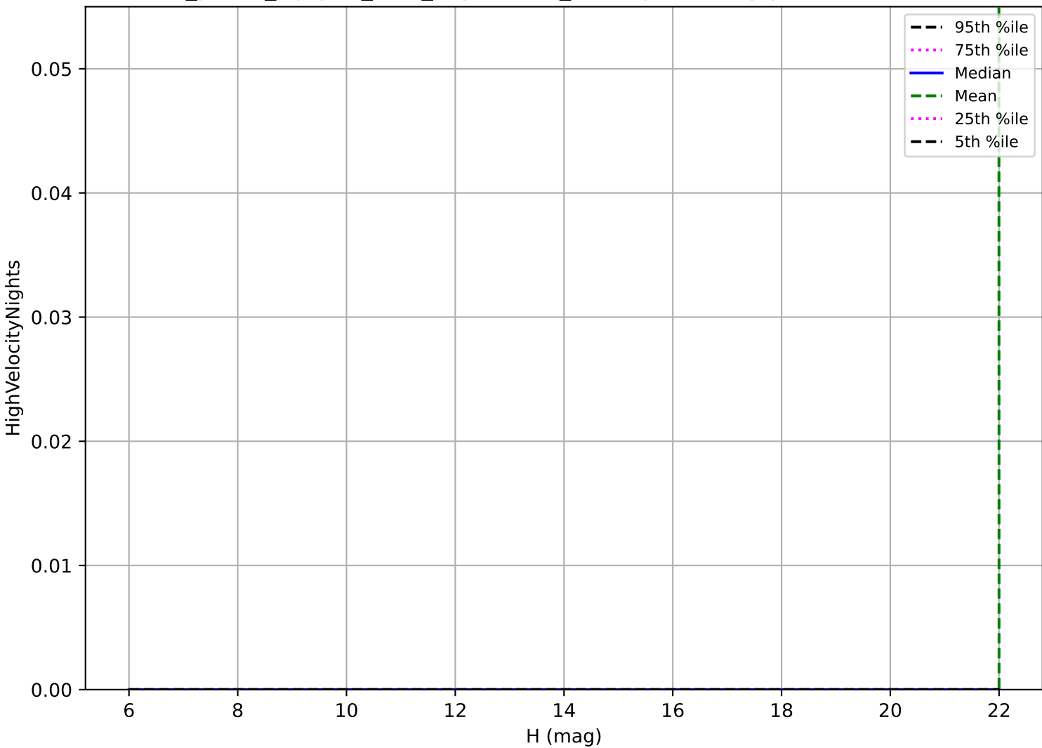
roll_pause_mjdp60_v3.4_10yrs: OCC_r20 High velocity pair detection loss
