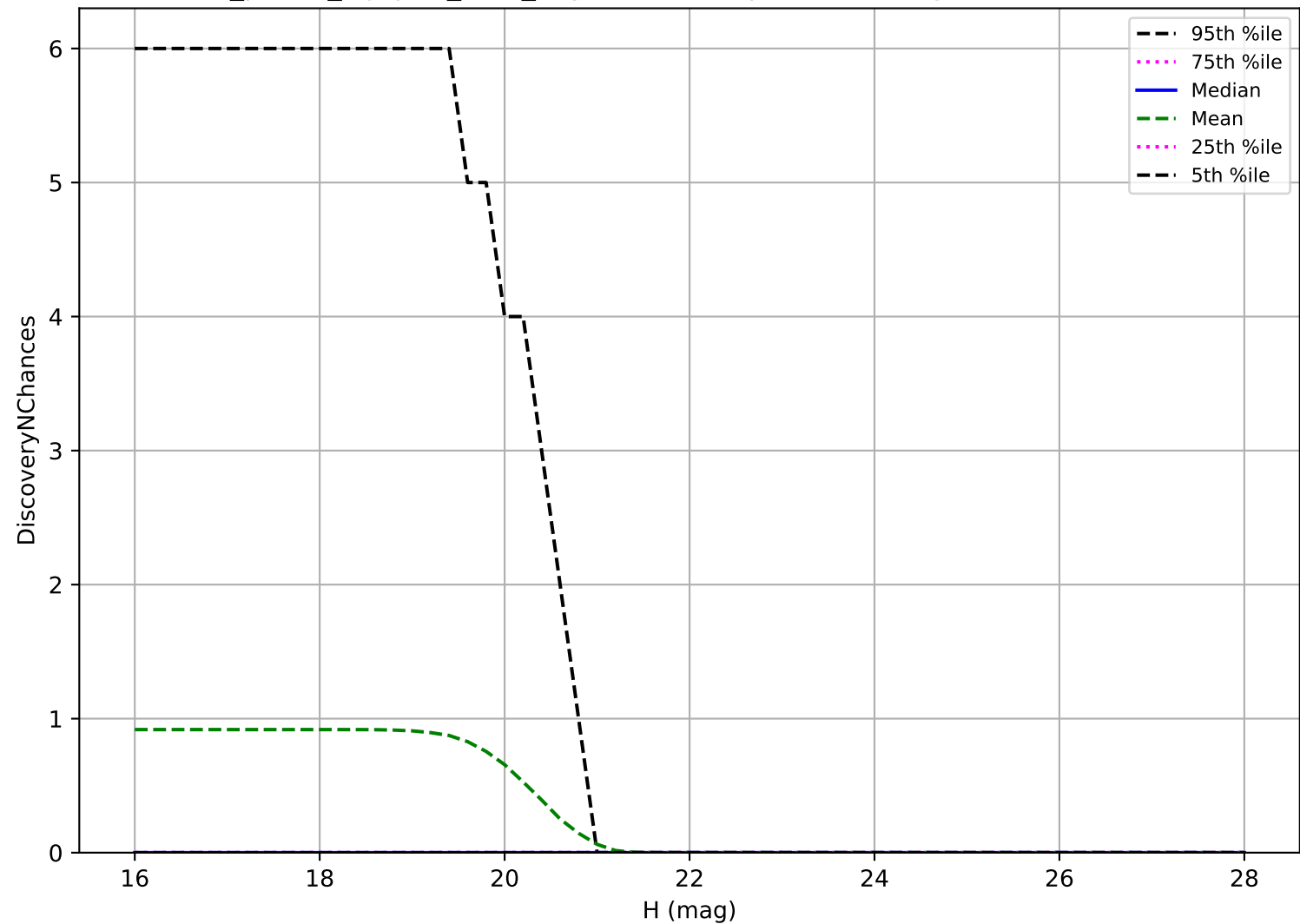
roll_pause_mjdp60_v3.4_10yrs: Vatira 3 pairs in 15 nights detection loss
