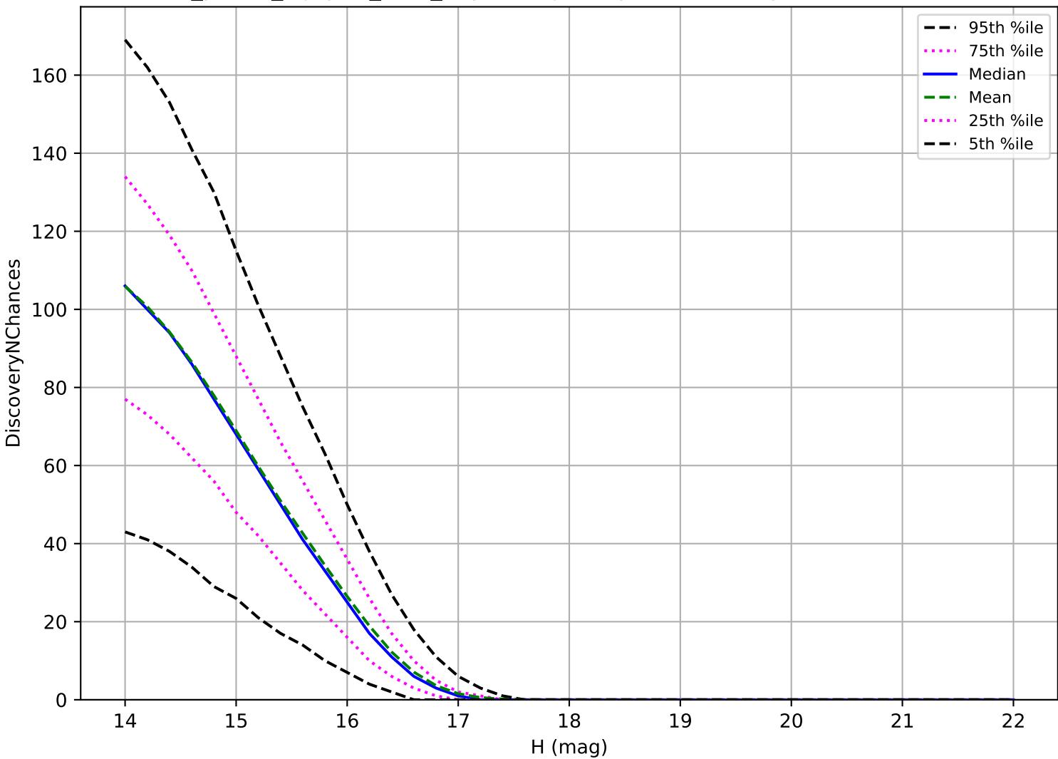
roll_pause_mjdp60_v3.4_10yrs: Trojan 3 pairs in 15 nights detection loss
