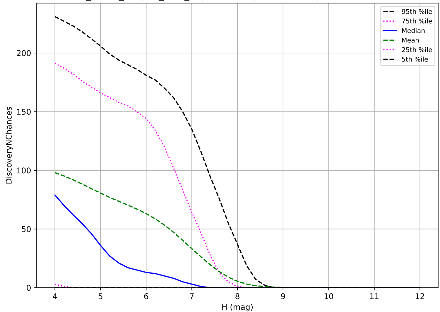
roll_pause_mjdp60_v3.4_10yrs: TNO 3 pairs in 15 nights detection loss
