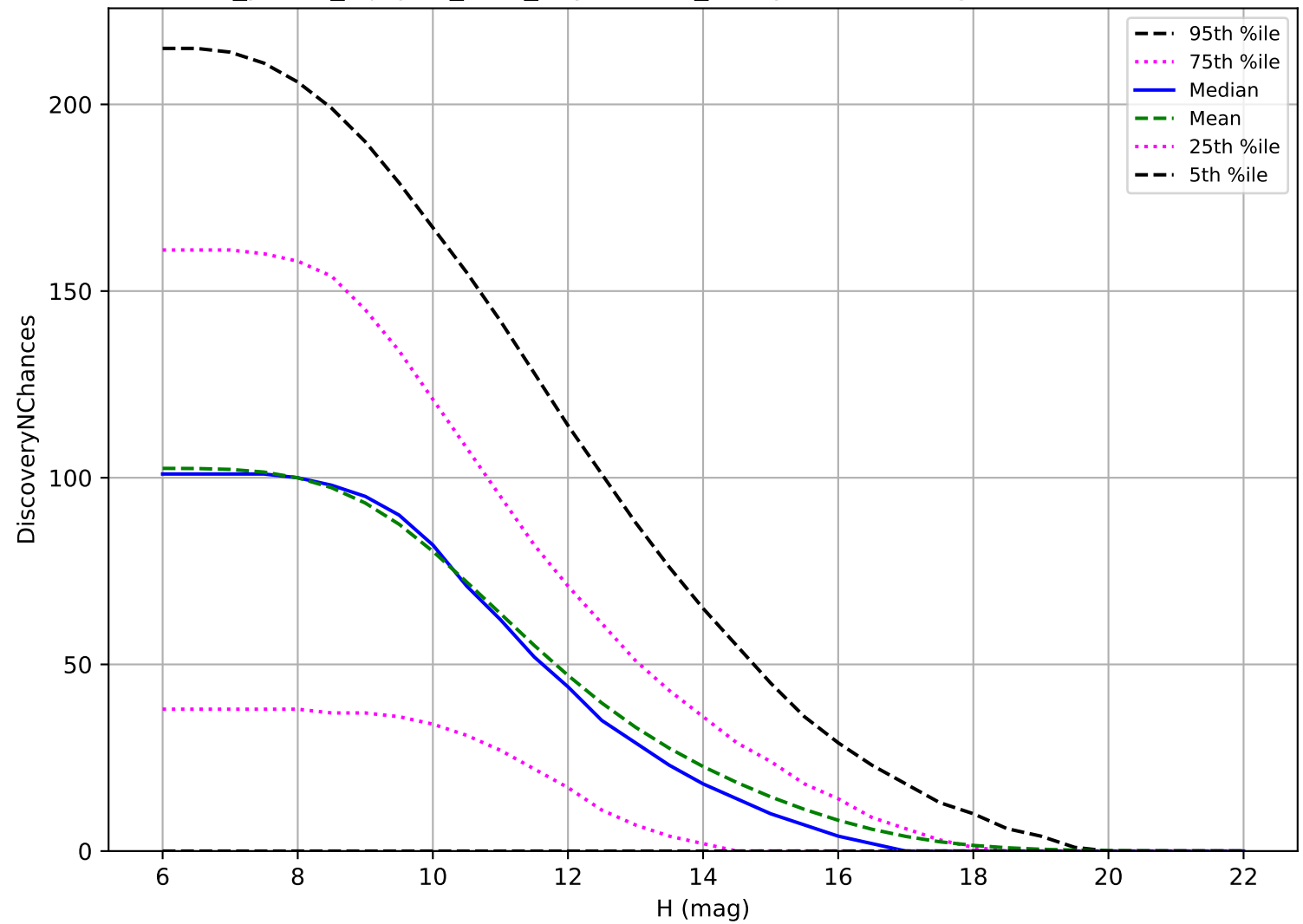
roll_pause_mjdp60_v3.4_10yrs: OCC_r5 3 pairs in 15 nights detection loss
