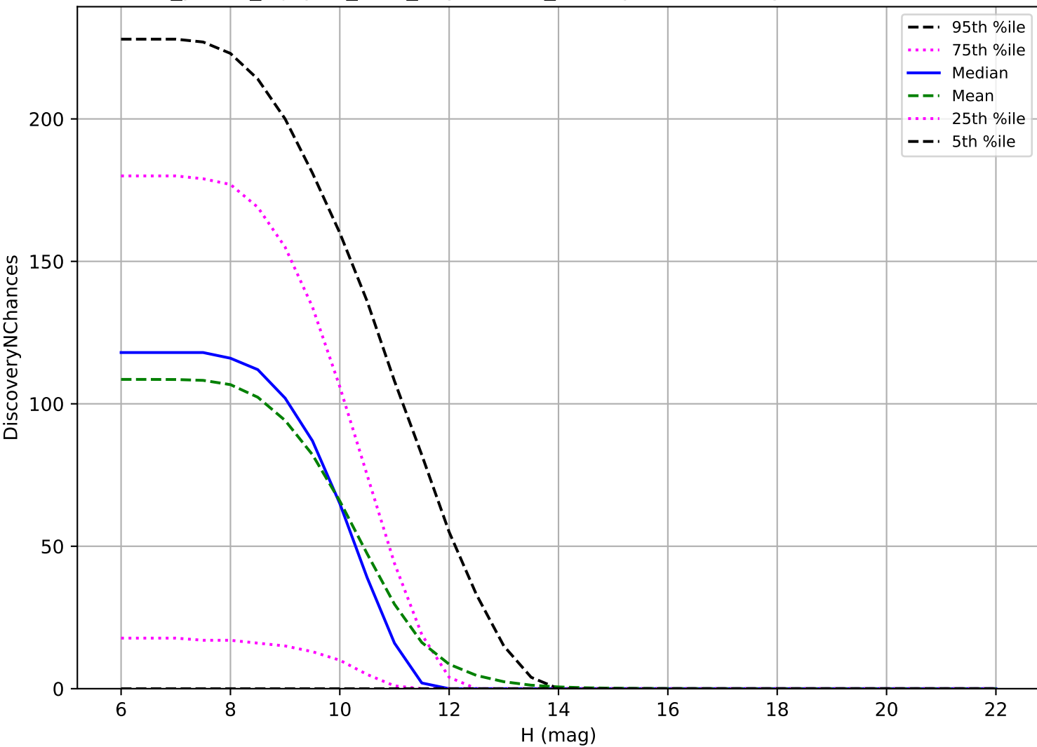
roll_pause_mjdp60_v3.4_10yrs: OCC_r20 3 pairs in 15 nights detection loss
