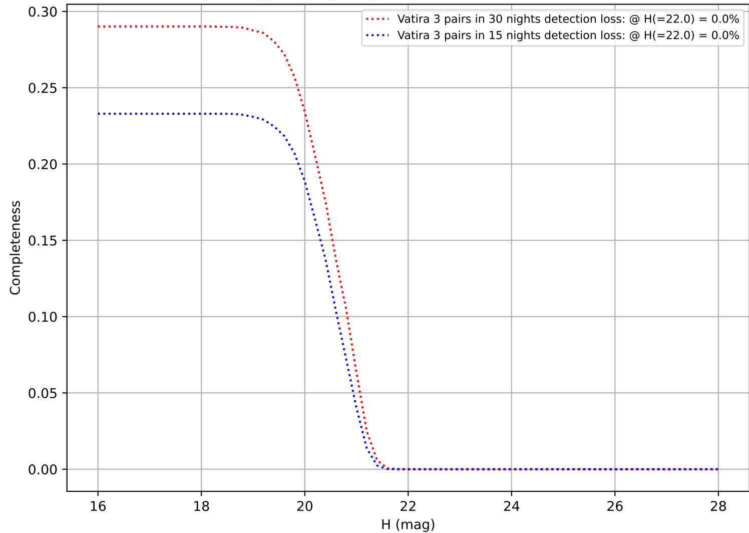
roll_pause_mjdp60_v3.4_10yrs: DifferentialCompleteness
