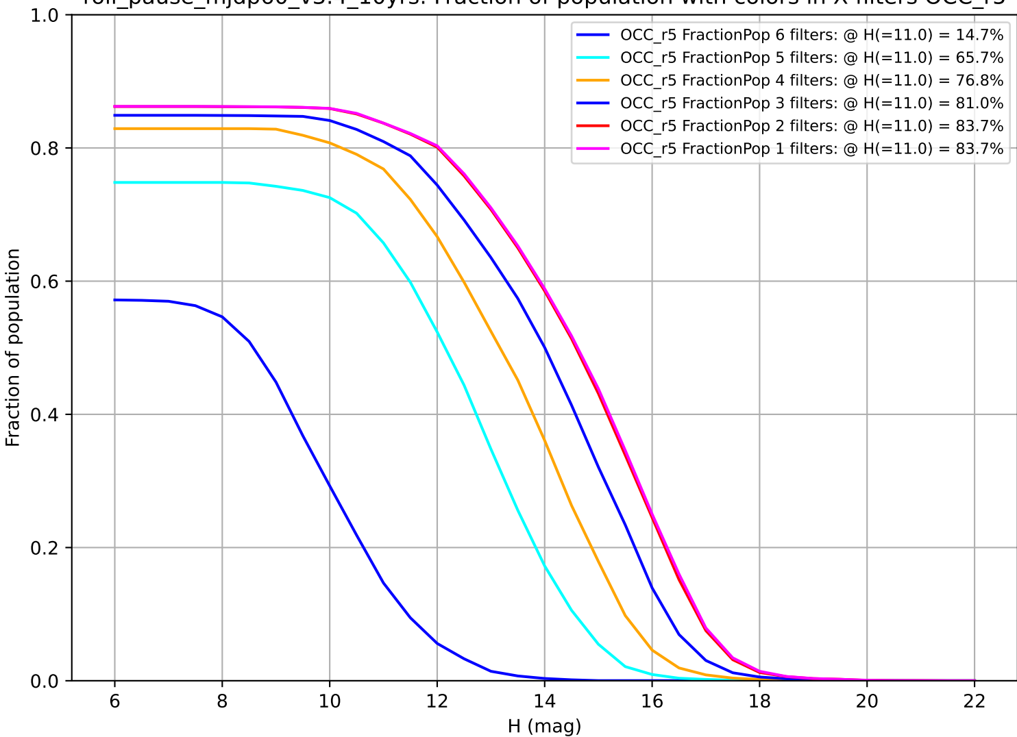
roll_pause_mjdp60_v3.4_10yrs: Fraction of population with colors in X filters OCC_r5
