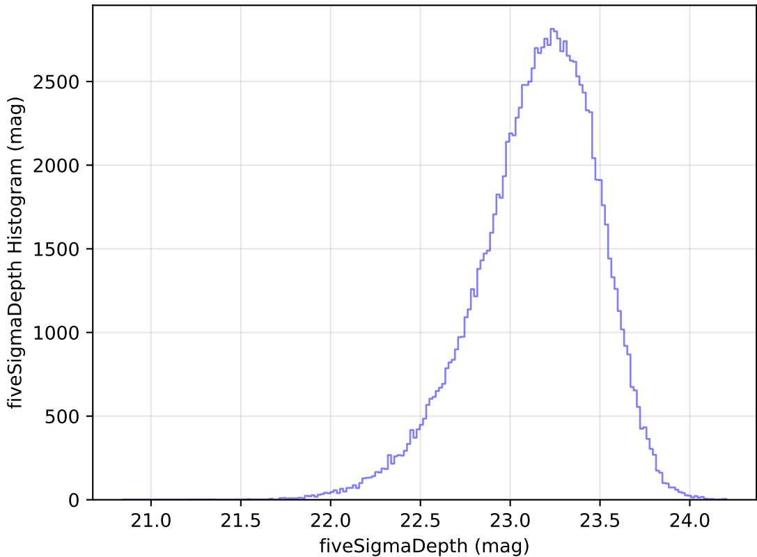
roll_pause_mjdp60_v3.4_10yrs u: fiveSigmaDepth Histogram
