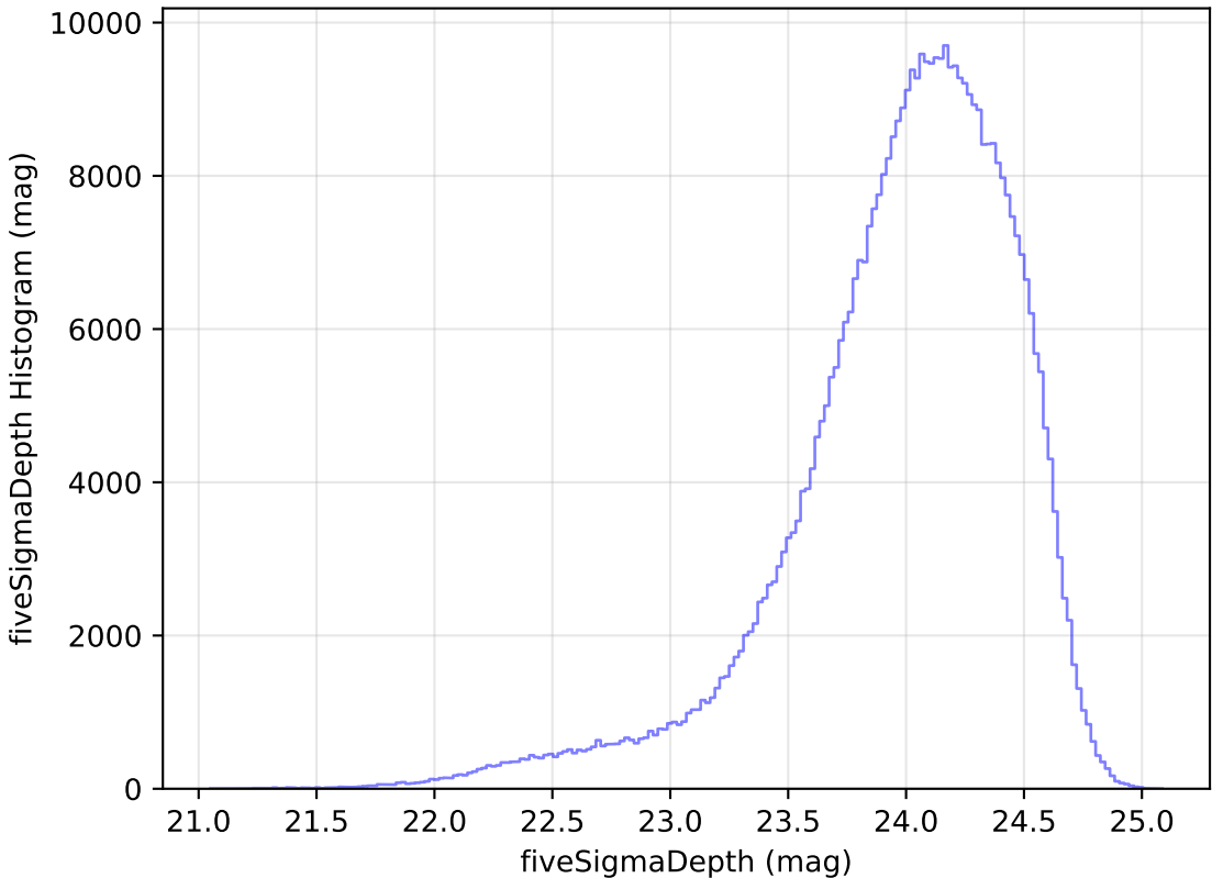
roll_pause_mjdp60_v3.4_10yrs r: fiveSigmaDepth Histogram
