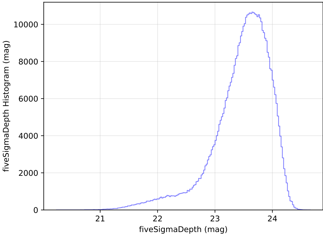
roll_pause_mjdp60_v3.4_10yrs i: fiveSigmaDepth Histogram
