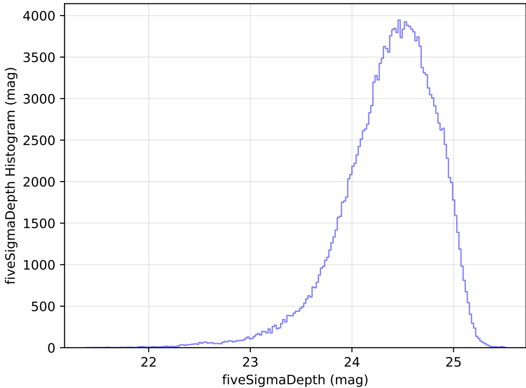
roll_pause_mjdp60_v3.4_10yrs g: fiveSigmaDepth Histogram
