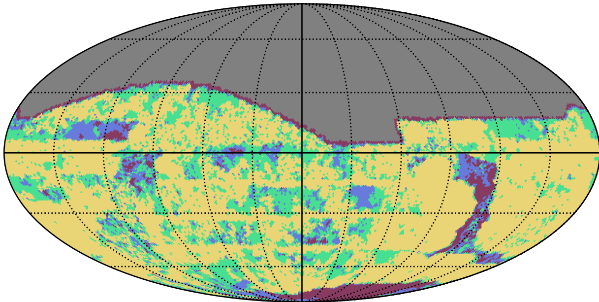
roll_pause_mjdp60_v3.4_10yrs g band: YearCoverage night
