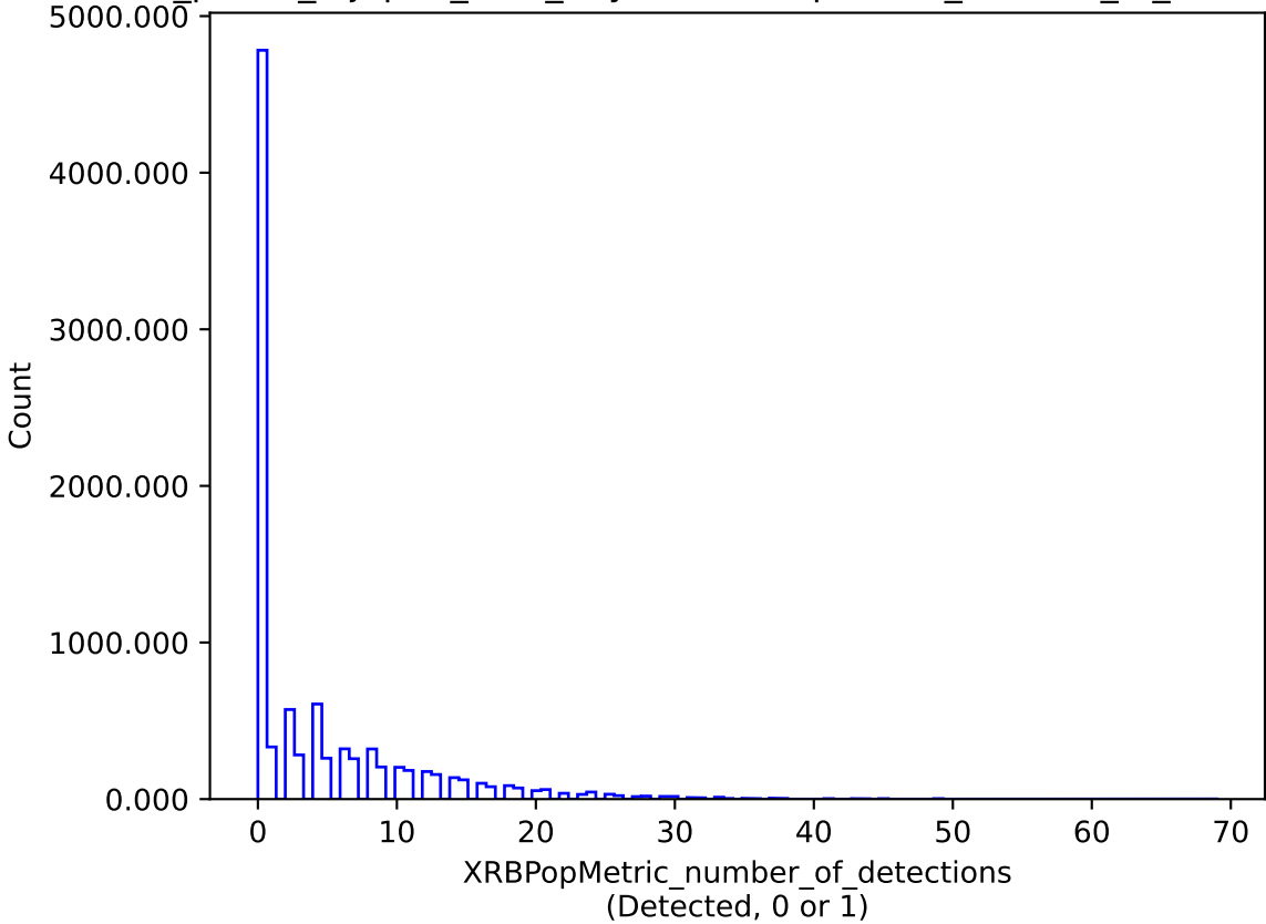
roll_pause_mjdp60_v3.4_10yrs : XRBPopMetric_number_of_detections
