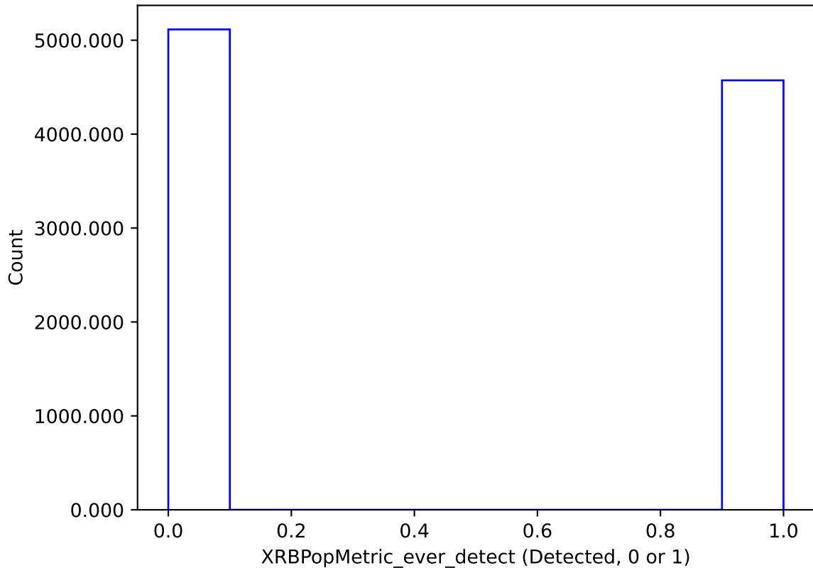
roll_pause_mjdp60_v3.4_10yrs : XRBPopMetric_ever_detect
