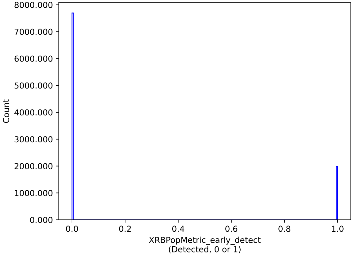
roll_pause_mjdp60_v3.4_10yrs : XRBPoMetric_early_detect
