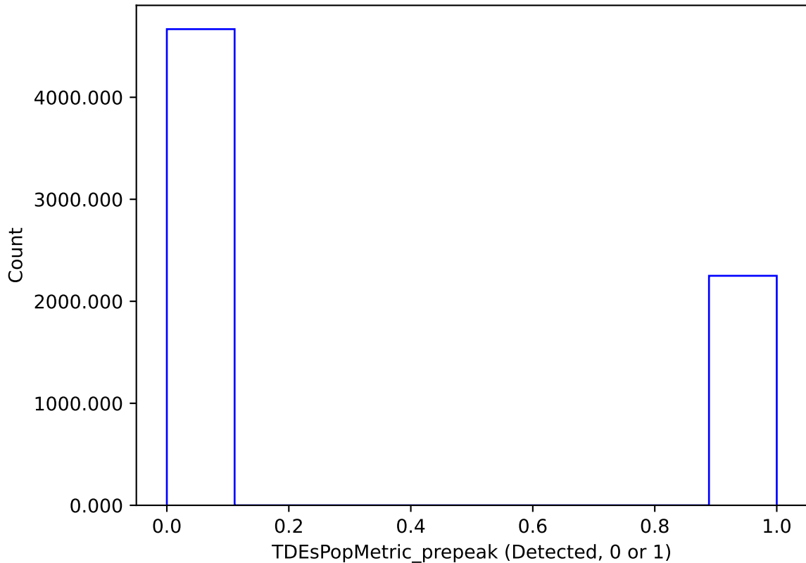
roll_pause_mjdp60_v3.4_10yrs : TDEsPopMetric_prepeak
