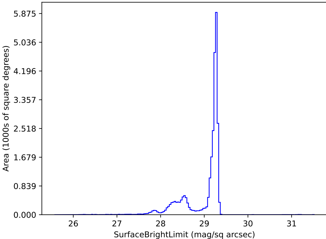
roll_pause_mjdp60_v3.4_10yrs z: SurfaceBrightLimit
