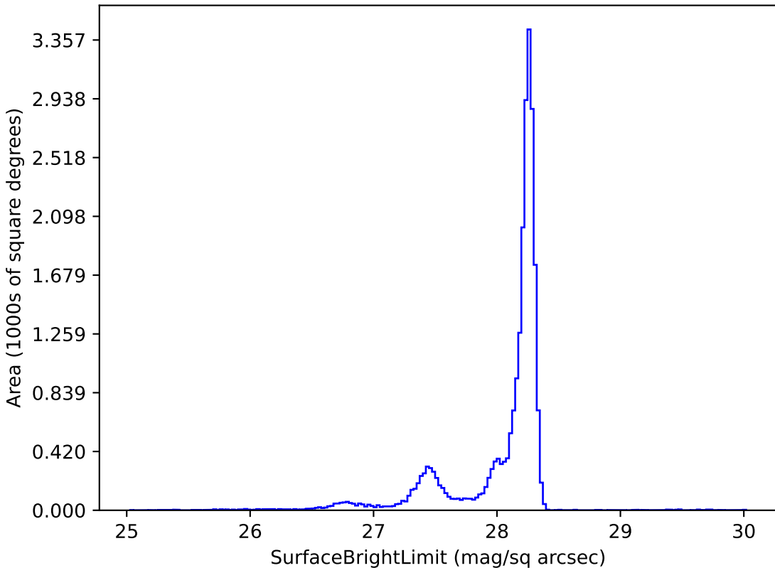
roll_pause_mjdp60_v3.4_10yrs y: SurfaceBrightLimit
