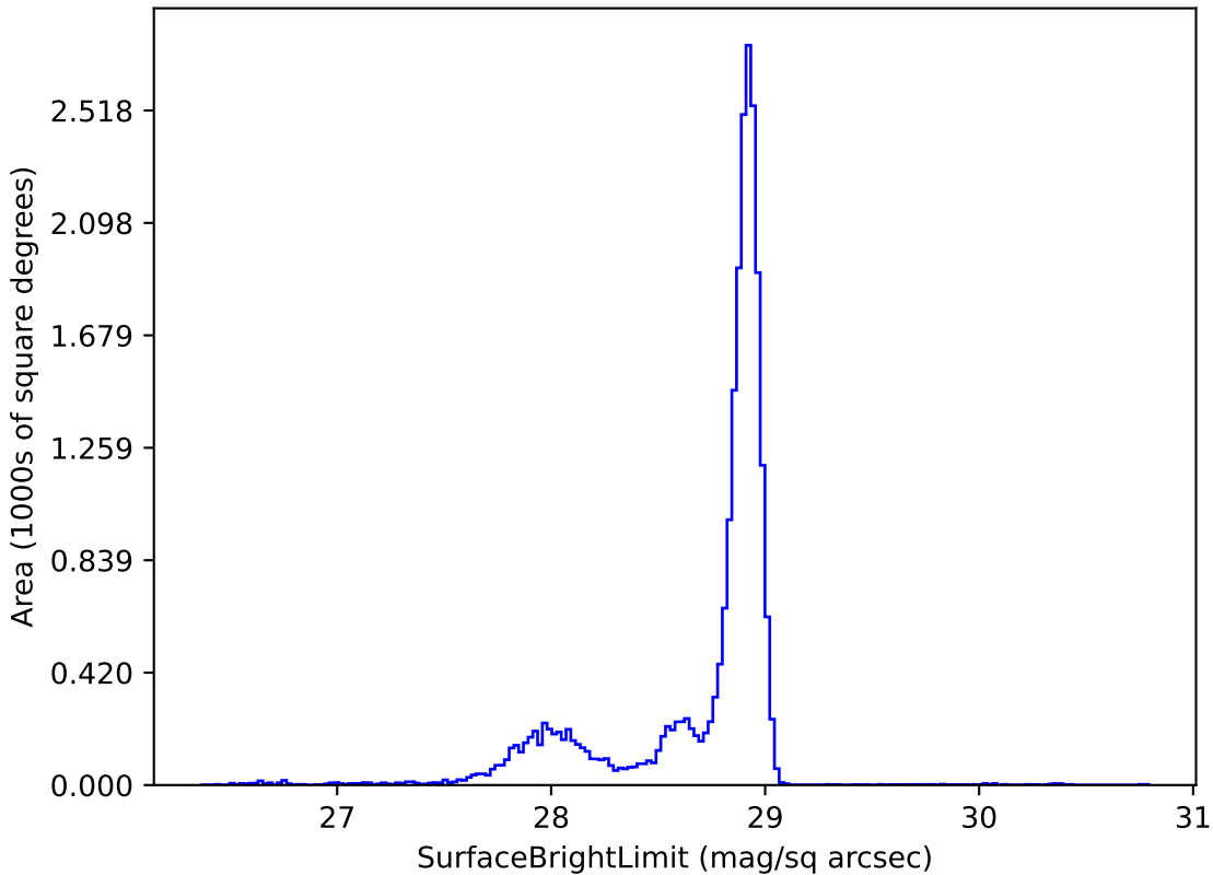
roll_pause_mjdp60_v3.4_10yrs u: SurfaceBrightLimit
