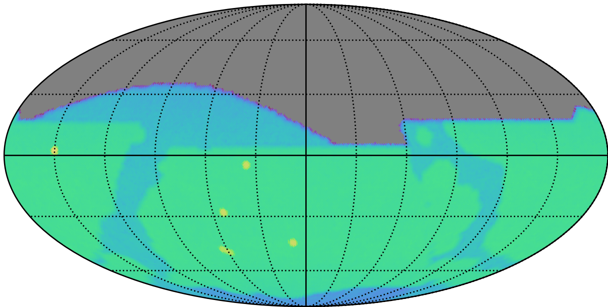
roll_pause_mjdp60_v3.4_10yrs i: SurfaceBrightLimit
