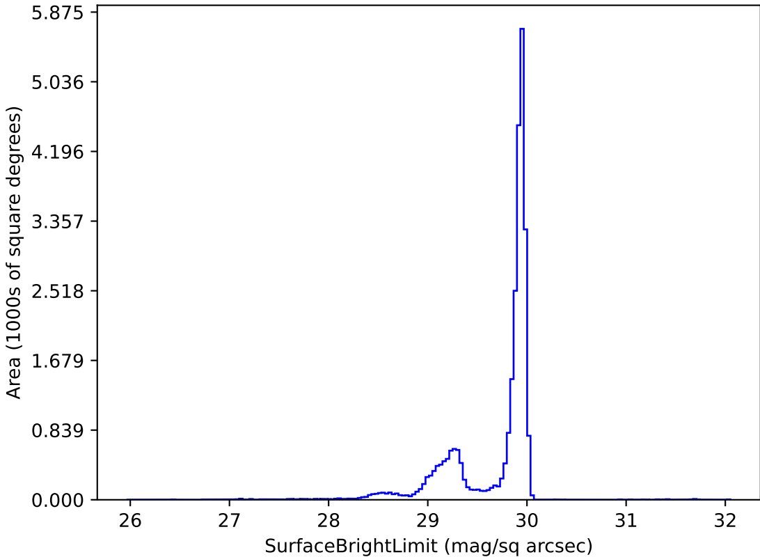
roll_pause_mjdp60_v3.4_10yrs i: SurfaceBrightLimit
