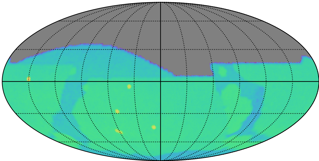
roll_pause_mjdp60_v3.4_10yrs g: SurfaceBrightLimit
