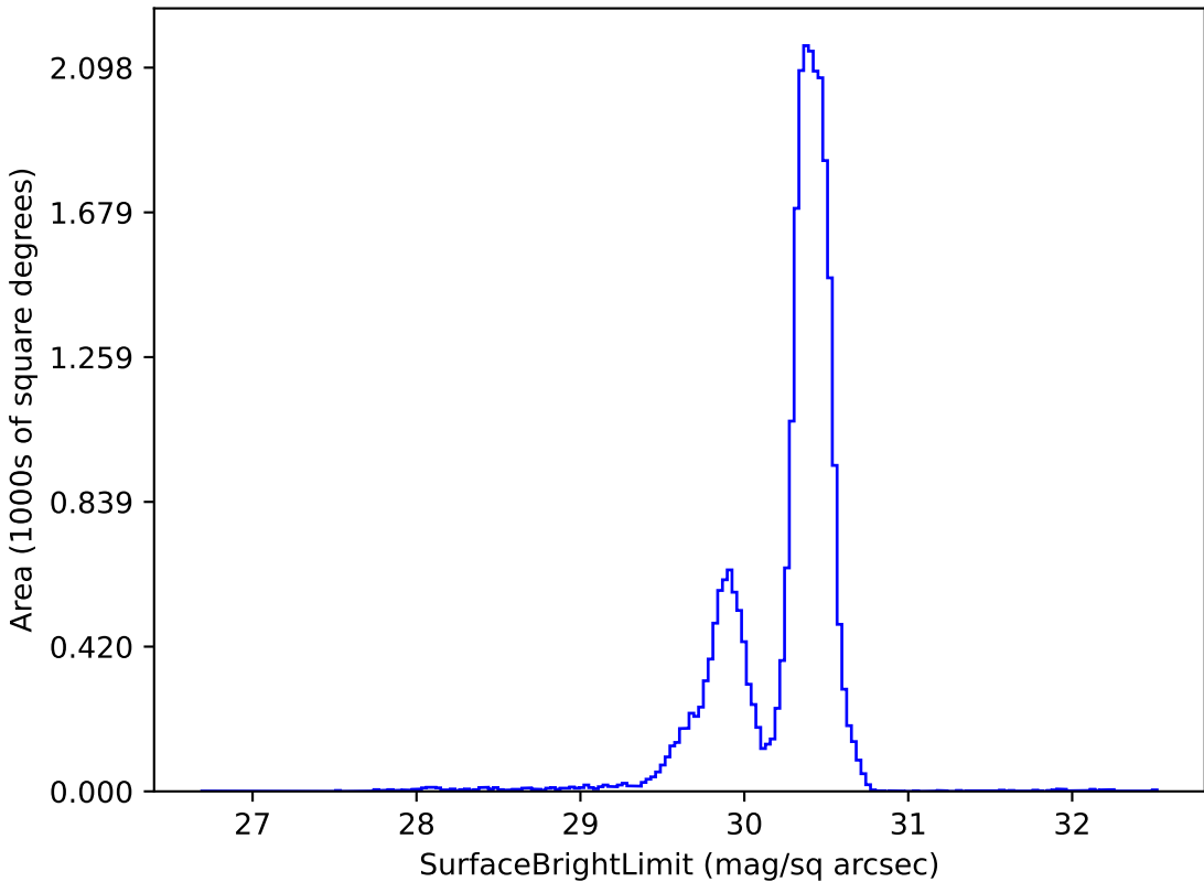
roll_pause_mjdp60_v3.4_10yrs g: SurfaceBrightLimit
