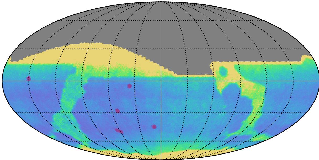
roll_pause_mjdp60_v3.4_10yrs : Proper Motion Uncert @ 24.0
