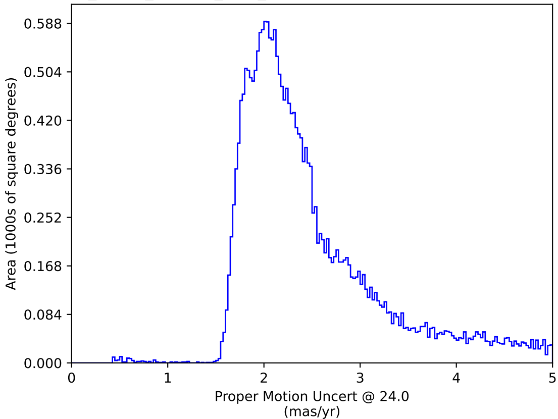
roll_pause_mjdp60_v3.4_10yrs : Proper Motion Uncert @ 24.0
