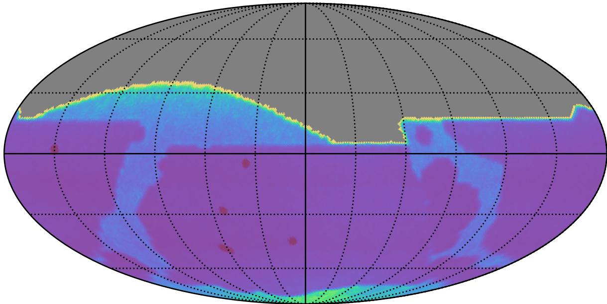
roll_pause_mjdp60_v3.4_10yrs : Proper Motion Uncert @ 20.5
