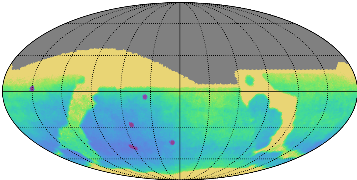
roll_pause_mjdp60_v3.4_10yrs : Parallax Uncert @ 24.0
