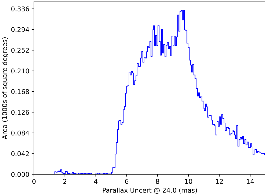
roll_pause_mjdp60_v3.4_10yrs : Parallax Uncert @ 24.0
