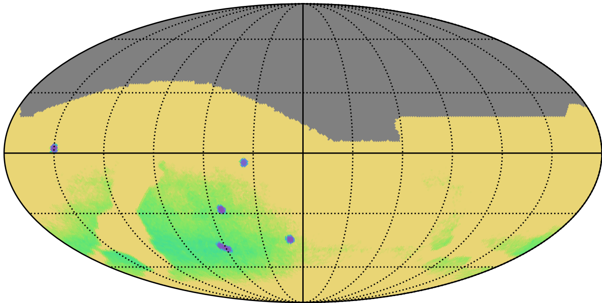
roll_pause_mjdp60_v3.4_10yrs : Parallax Uncert @ 22.4
